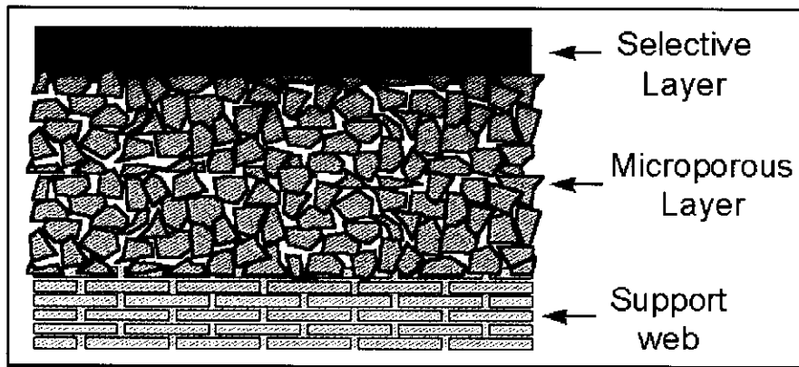
Figure 1 The three-layer VaporStep membrane
