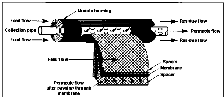
Figure 2 How the membrane is packaged into a spiral-wound module
